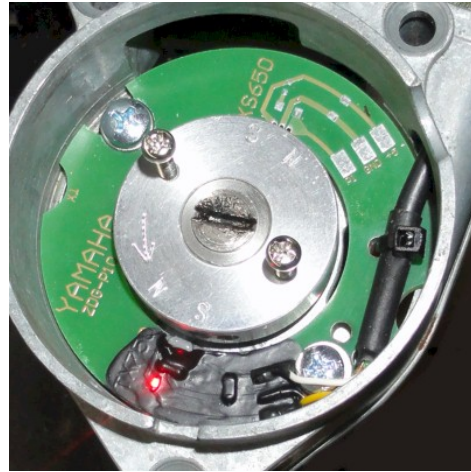
Figure 6 The LED goes on when the S-magnet passes the sensor and off when the N-magnet passes the sensor.
