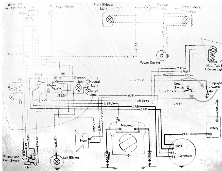
Figure 2 Original wiring diagram R69S.
