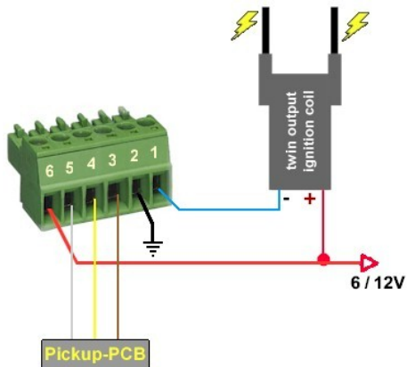
Ignition circuit diagram with one 6 V dual output coil.
