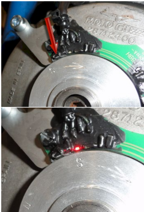
Figure 5 Adjust the magnet disk so that the LED just goes from on to off.
