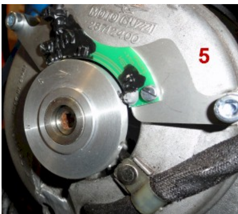
Magnet disk installation
