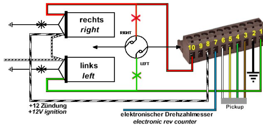
Figure 3 Ignition circuit diagram, breaker points replacement
