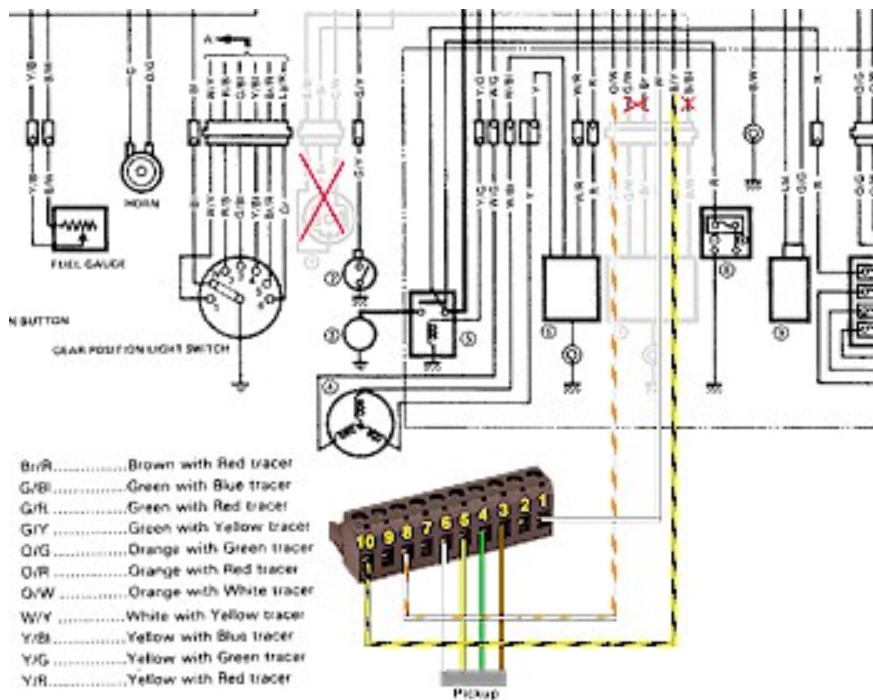
Figure 3 Circuit diagram.
