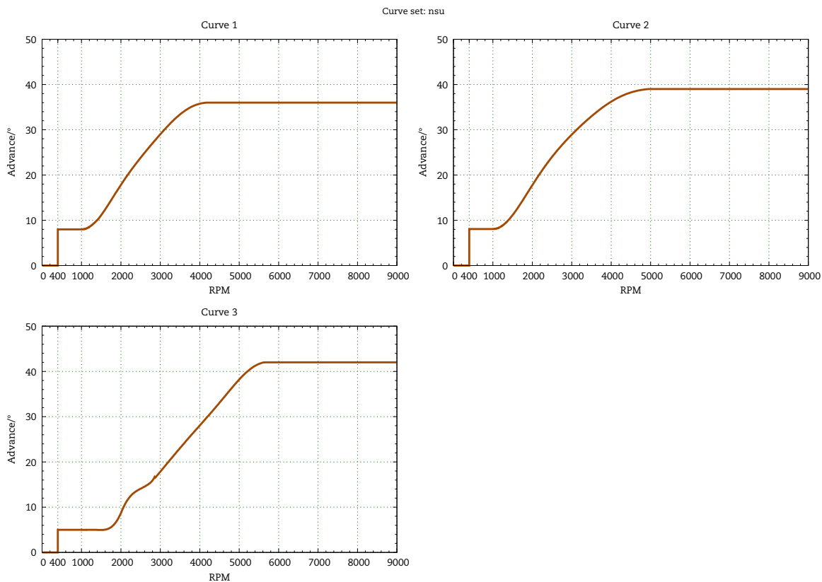
Figure 8 Selectable ignition curves.
