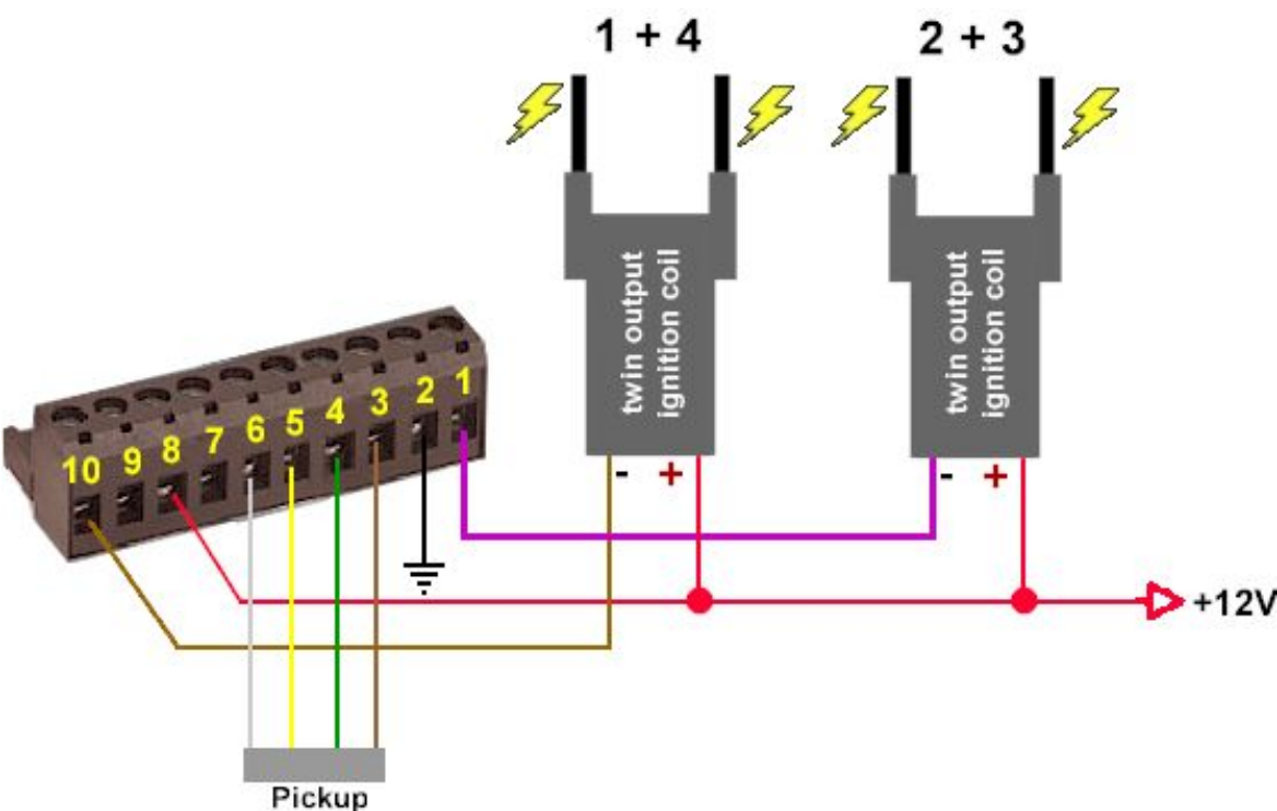
Ignition circuit diagram
