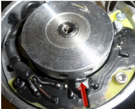
Figure 3 Ensure correct alignment of magnet disk and sensor.
