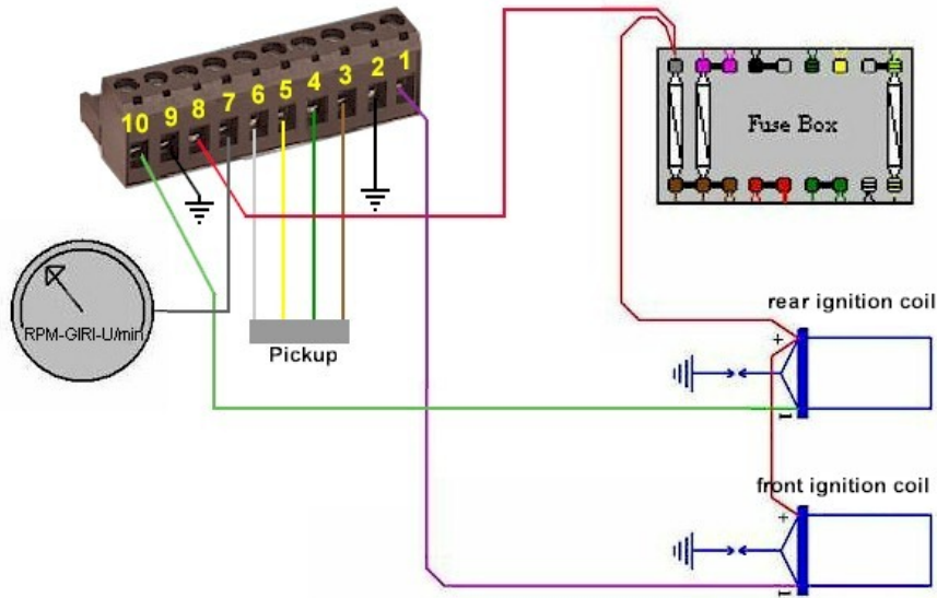
Figure 3 Circuit diagram.
