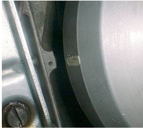
Figure 6.a Set the rear piston to TDC.
