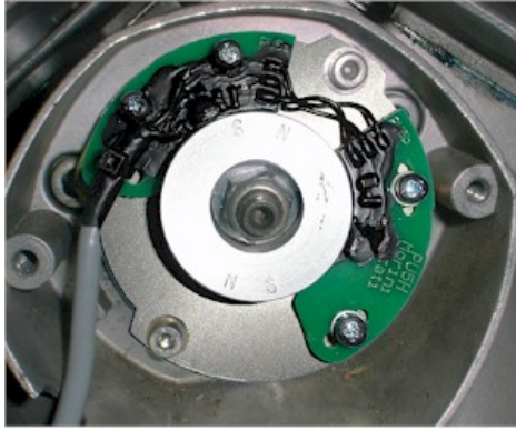
Figure 2 Assembly of the pickup
