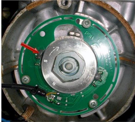
Figure 8.a This sensor is used for the initial setup.
