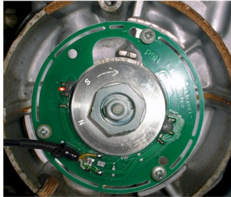
Figure 8.b The LED turns on when the S-magnet passes the sensor.
