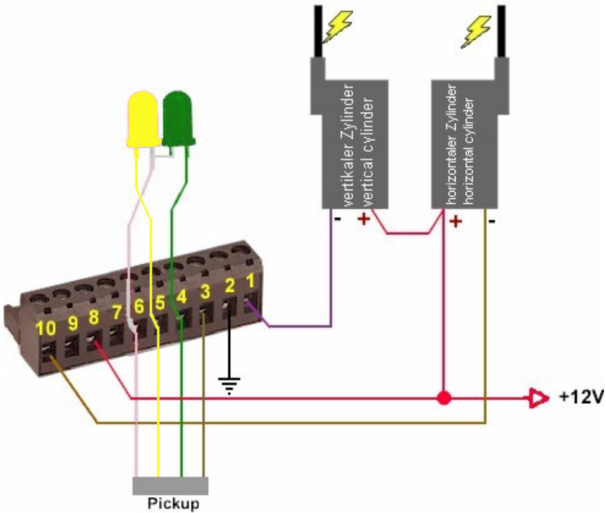
Ignition circuit diagram, also connect the test LEDs for the later setting
